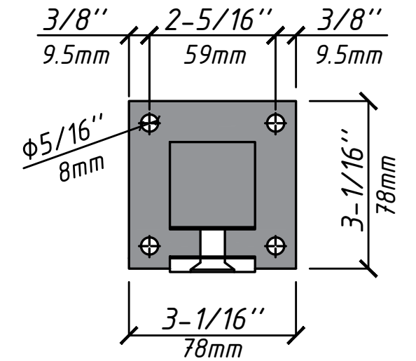
CG1207 BOTTOM VIEW
