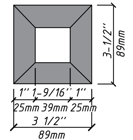
COVER FOR BASE PLATE
