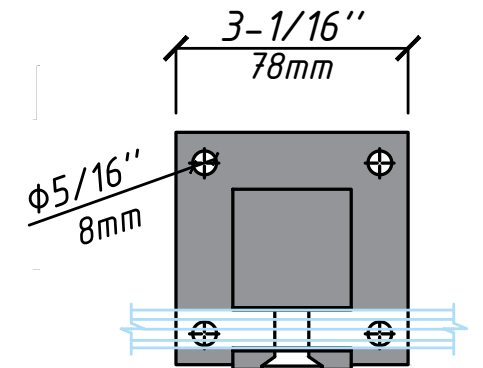
CG1207 TOP VIEW
